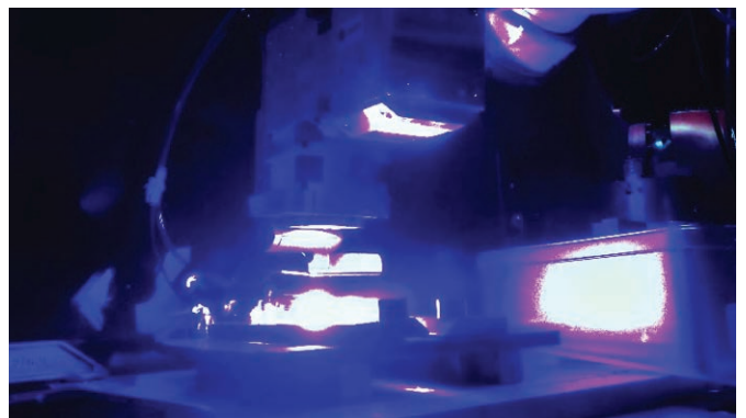
© Fraunhofer USA Center for Laser Applications CLA, Laser beam welding of copper using new Blue laser source
