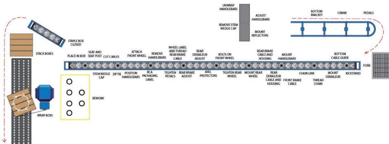
© Fraunhofer USA, The BCA Project Team analyzed bike assembly workflow, pinpointed inefficiencies and built the architecture and cloud-based platform for manufacturing knowledge capture
