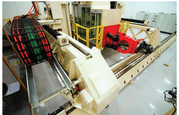
AFP Project researchers are using the Ingersoll LYNX Automated Fiber Placement Machine housed at the University of South Carolina's McNair Center as the testbed
